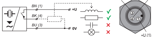
Connection diagram of the ULS sensor with P type output (PNP) with an open collector
