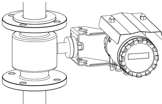
Mounting flowmeter in vertical pipe
