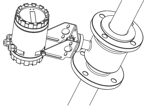
Mounting flowmeter in upward pipe
